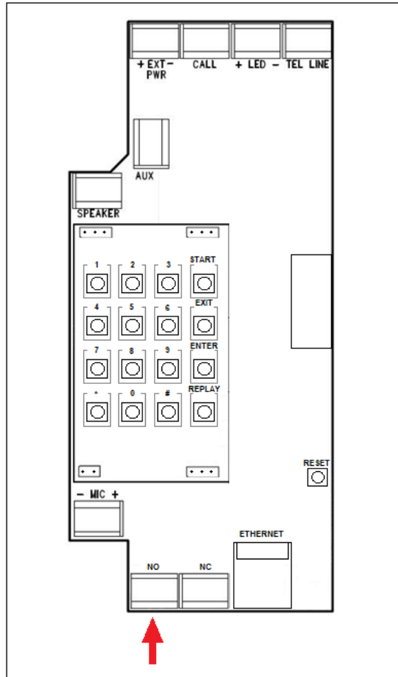
Figure 1- MWP-302 NO Dry contact.
